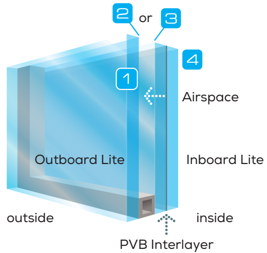
DOUBLE GLAZING IGU WITH LAMINATED GLASS
