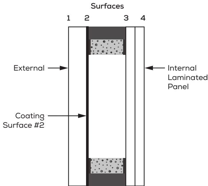
FIG.4 IGU LAMINATED
