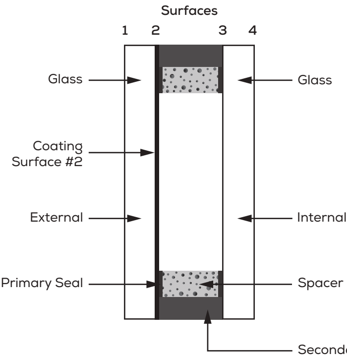
FIG.3 IGU LOW-E
